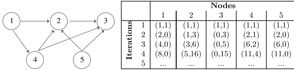
Figure 3: Example graph and the accompanying first iterations of the HITS webmining algorithm.
