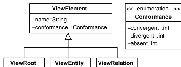
Fig. 4. Generic metamodel elements
