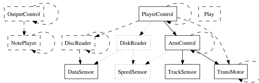
Fig. 5. Merged MADL conformance model
