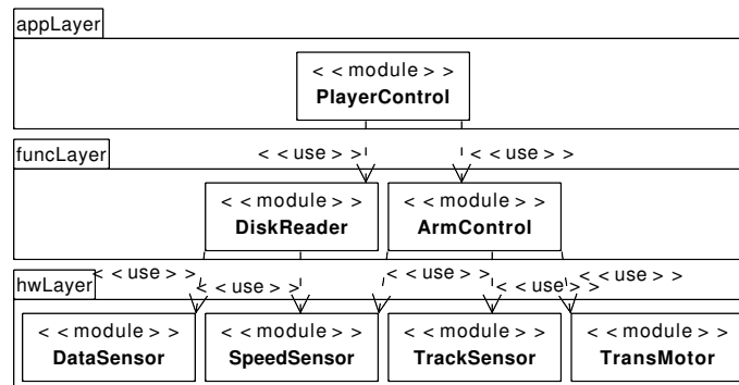
Fig. 1. Module-uses view
