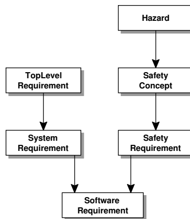
Fig. 6. Information model for the requirements engineering phase.
