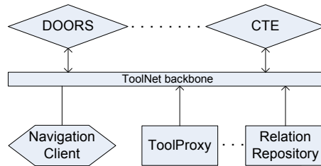
Fig. 5. ToolNet Architecture.
