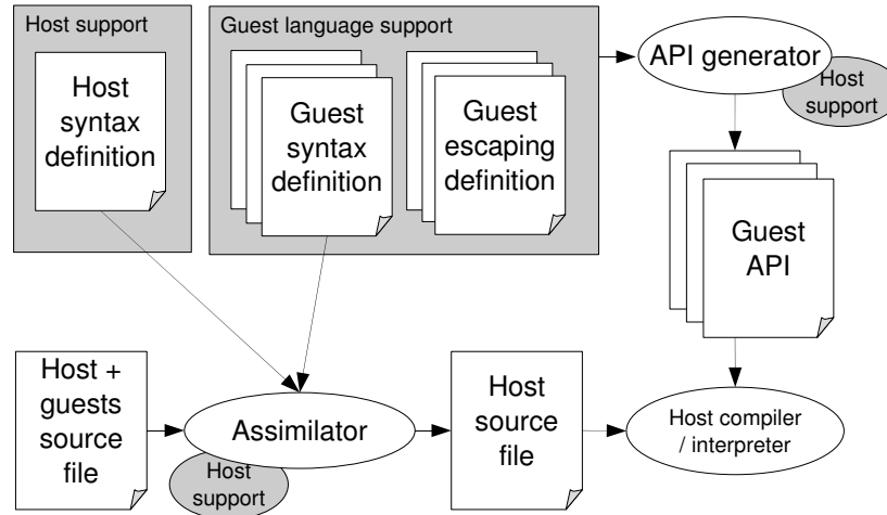
Figure 3: Overview of the StringBorg approach
